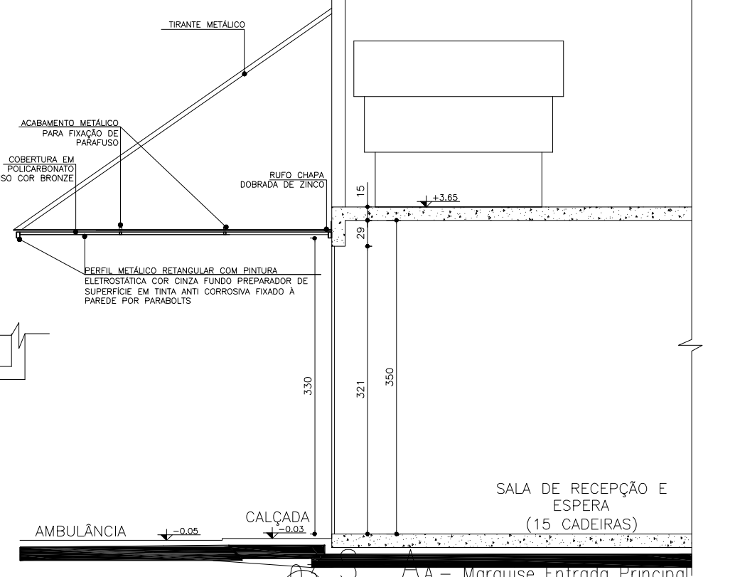
07 S AA'-Marquise Entrada Principal
